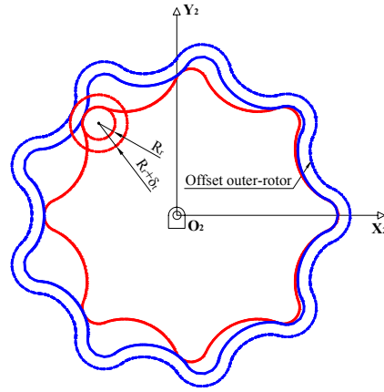
Fig. 4. Equidistant offset outer-rotor lobe profile (dashed line).
